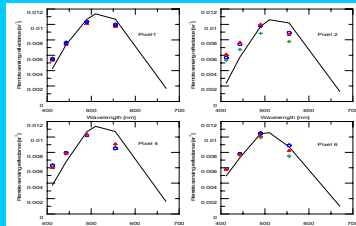
Figure 10. Examples of SeaWiFS estimated remote sensing reflectance spectra (solid lines) and in-situ measured remote sensing reflectance (crosses, triangles and circles) for selected pixels of sub-pixel variability experiment.
